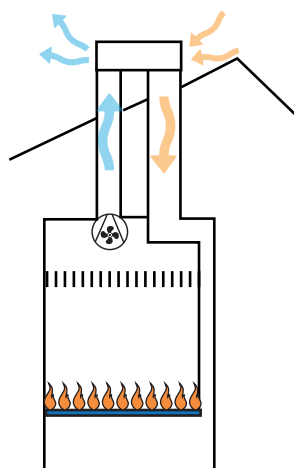
TYPE C32
