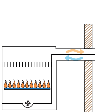
TYPE C13
