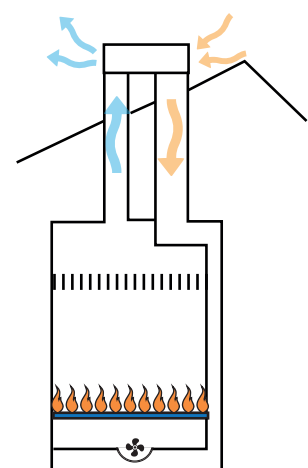
TYPE C33
