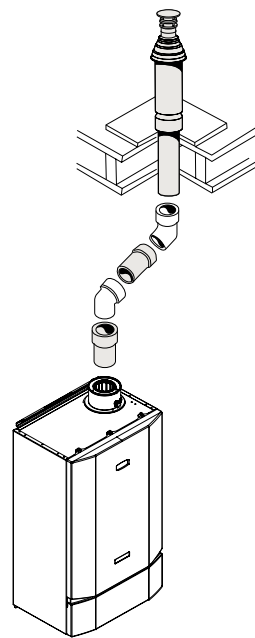
EXAMPLE 3 (OPEN FLUE)
